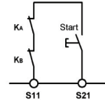
Fig. 8: Feedback loop for monitored manual start: The feedback loop monitors contactors or the expansion modules.
