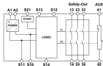
Fig. 1 Block diagram SCR-3
